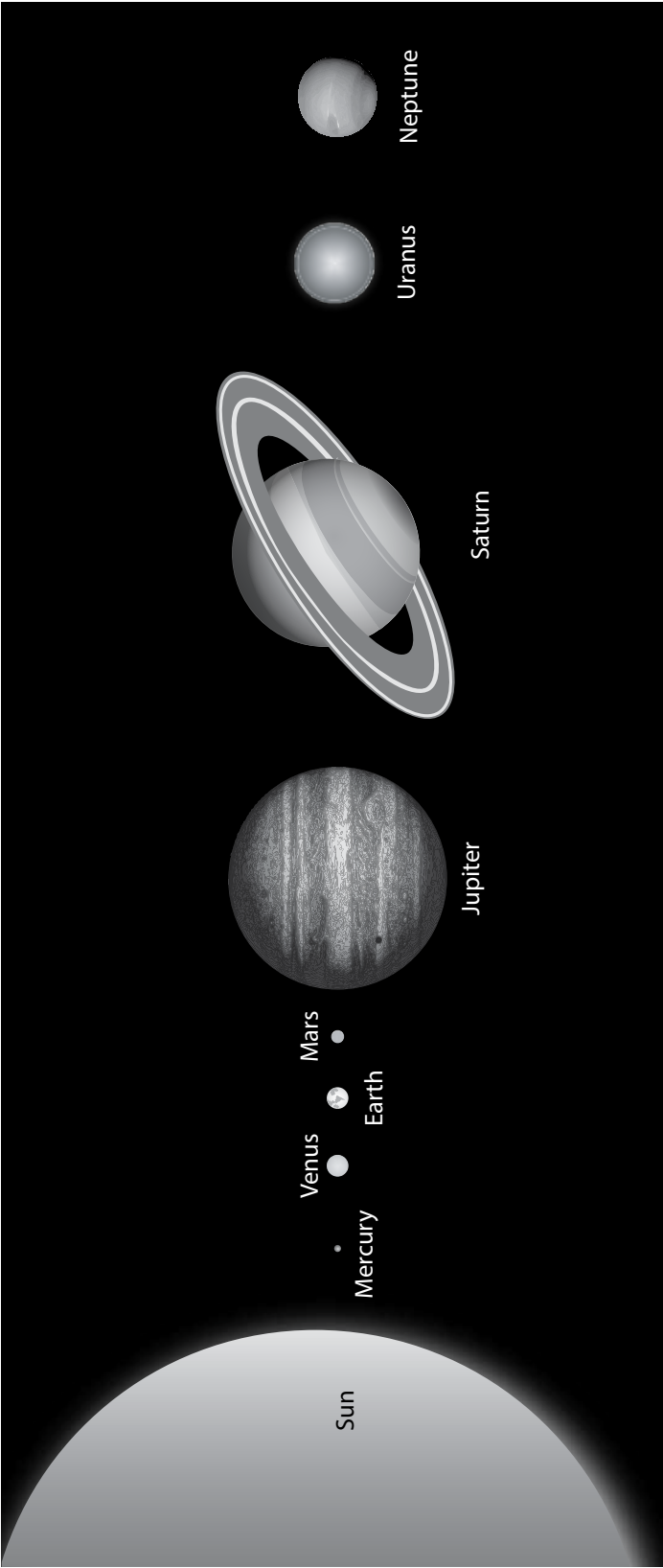
The Solar System
